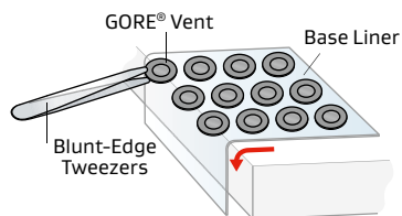
Figure 2: Manually dispensing an Adhesive Vent
