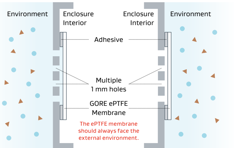
Figure 7: Interior or exterior mounting is recommended for Parts Series VE7 and VE9
