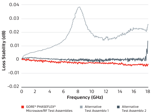
Figure 3: Loss Stability with Flexure of New Cables
