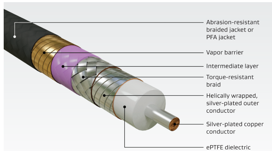
Figure 1: Rugged Construction
