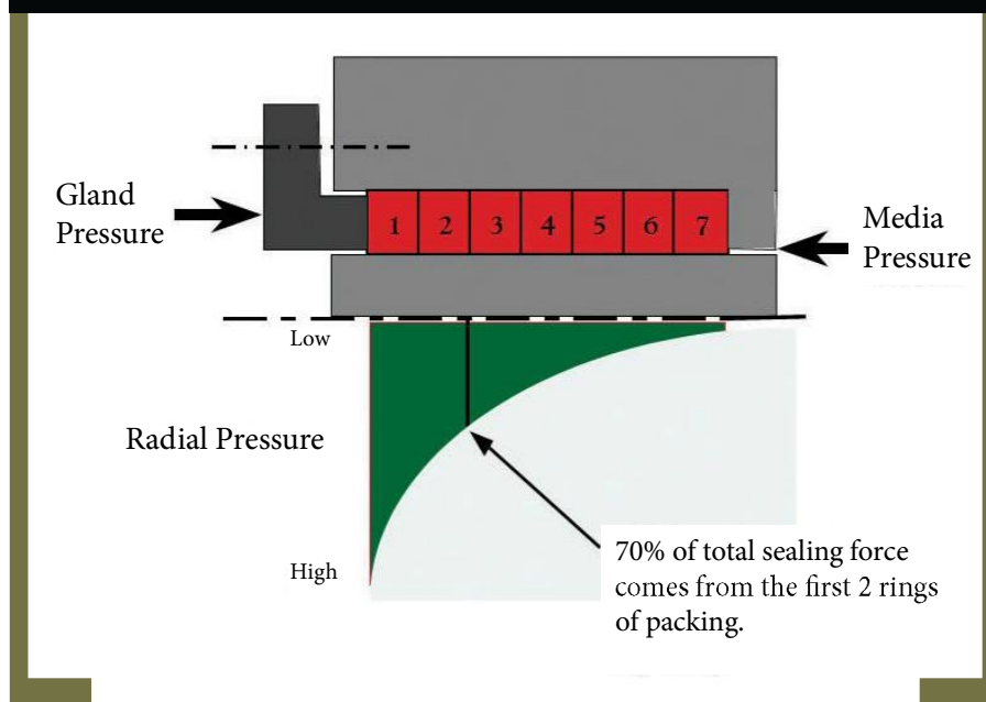
Figure 2. Stuffing box radial pressure distribution
