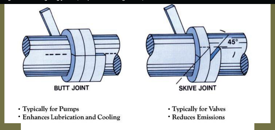
Figure 1. Packing ring joints (Graphics courtesy of FSA)
