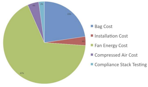
Figure 2. TCO for a pulse jet cement kiln baghouse using GORE® low drag filter bags.
