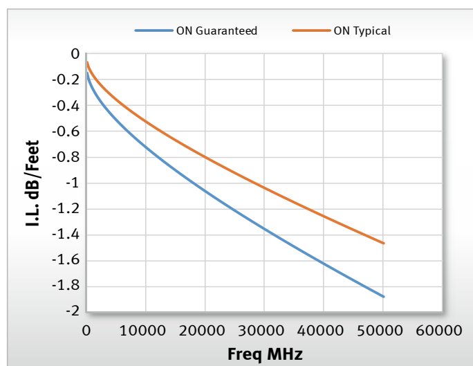
Figure 2: Gore Cable Type 0N Insertion Loss
