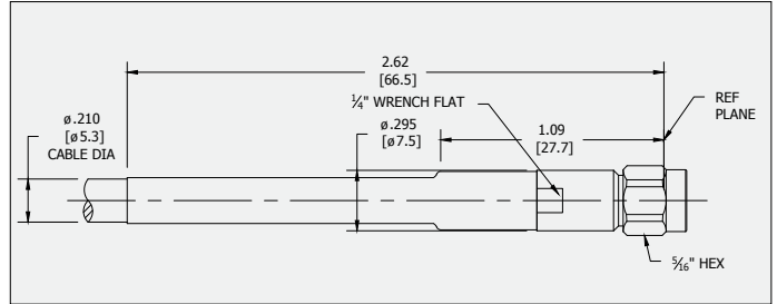
Figure 5: 2.92 mm (Male and Female)
