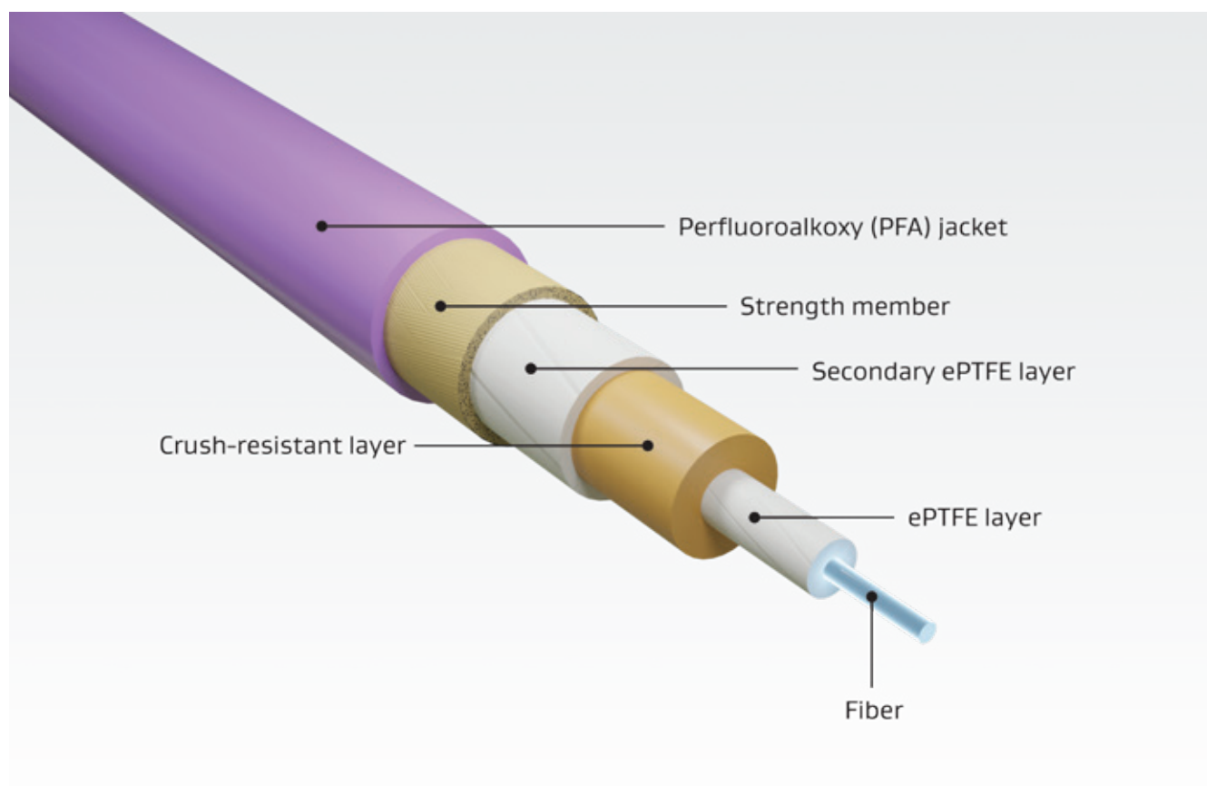
Figure 40: Crush-Resistant Layers
