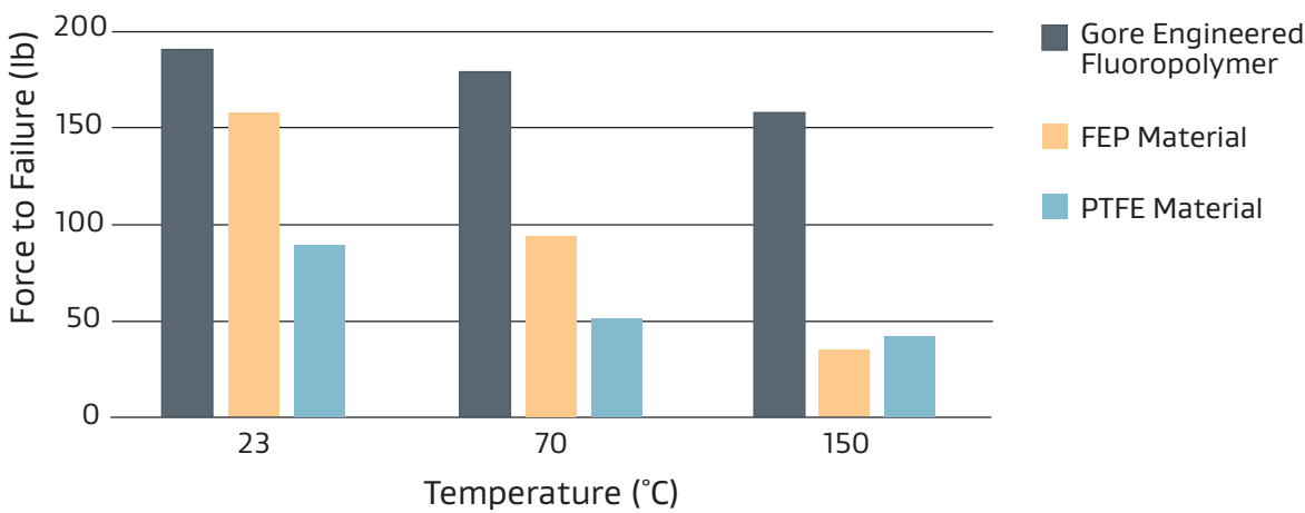
Figure 1: Cut-Through Resistance at High Temperatures
