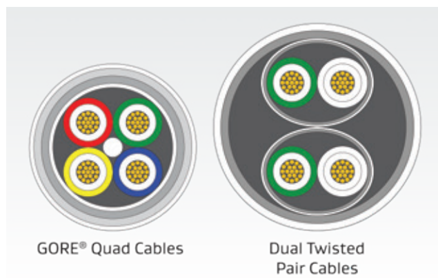
Figure 23: Reduced Cable Design
