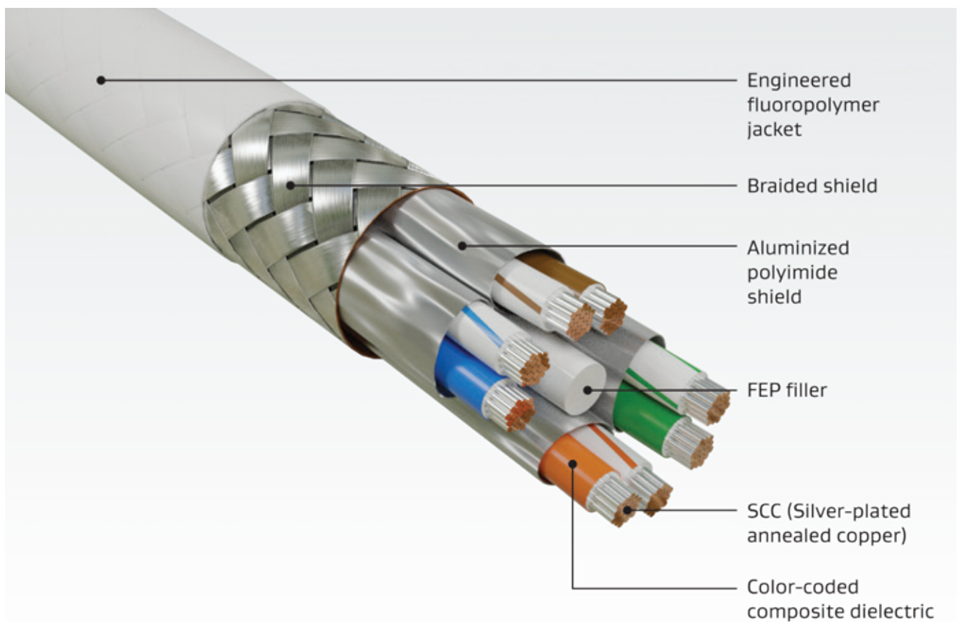
Figure 8: High-Density Construction
