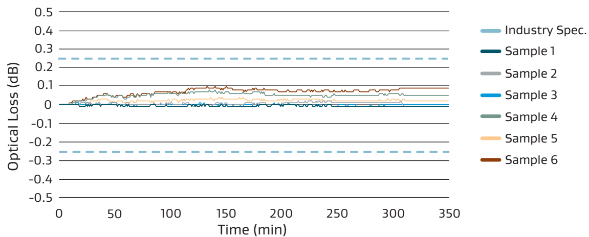
Figure 46: Vibration Endurance at +135°C (1300 nm)
