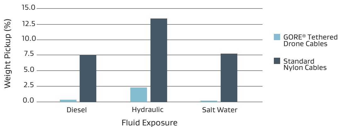
Figure 54: Comparison of Weight Stability After Fluid Immersion
