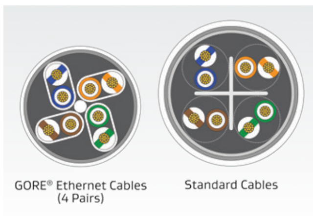
Figure 9: Reduced Diameter
