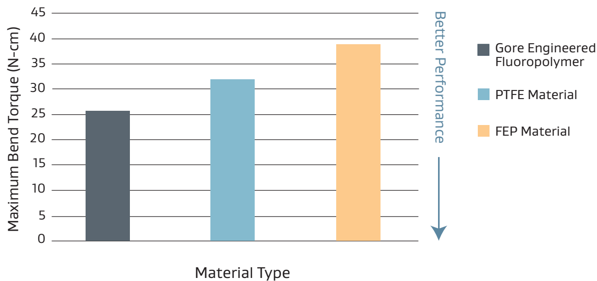
Figure 2: Flexure Comparison
