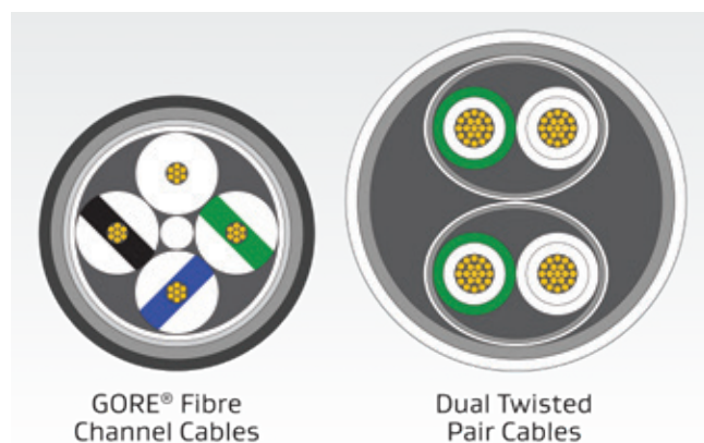
Figure 31: Low-Dielectric Cable Geometry
