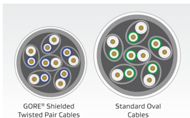
Figure 4: Low-Profile Configuration
