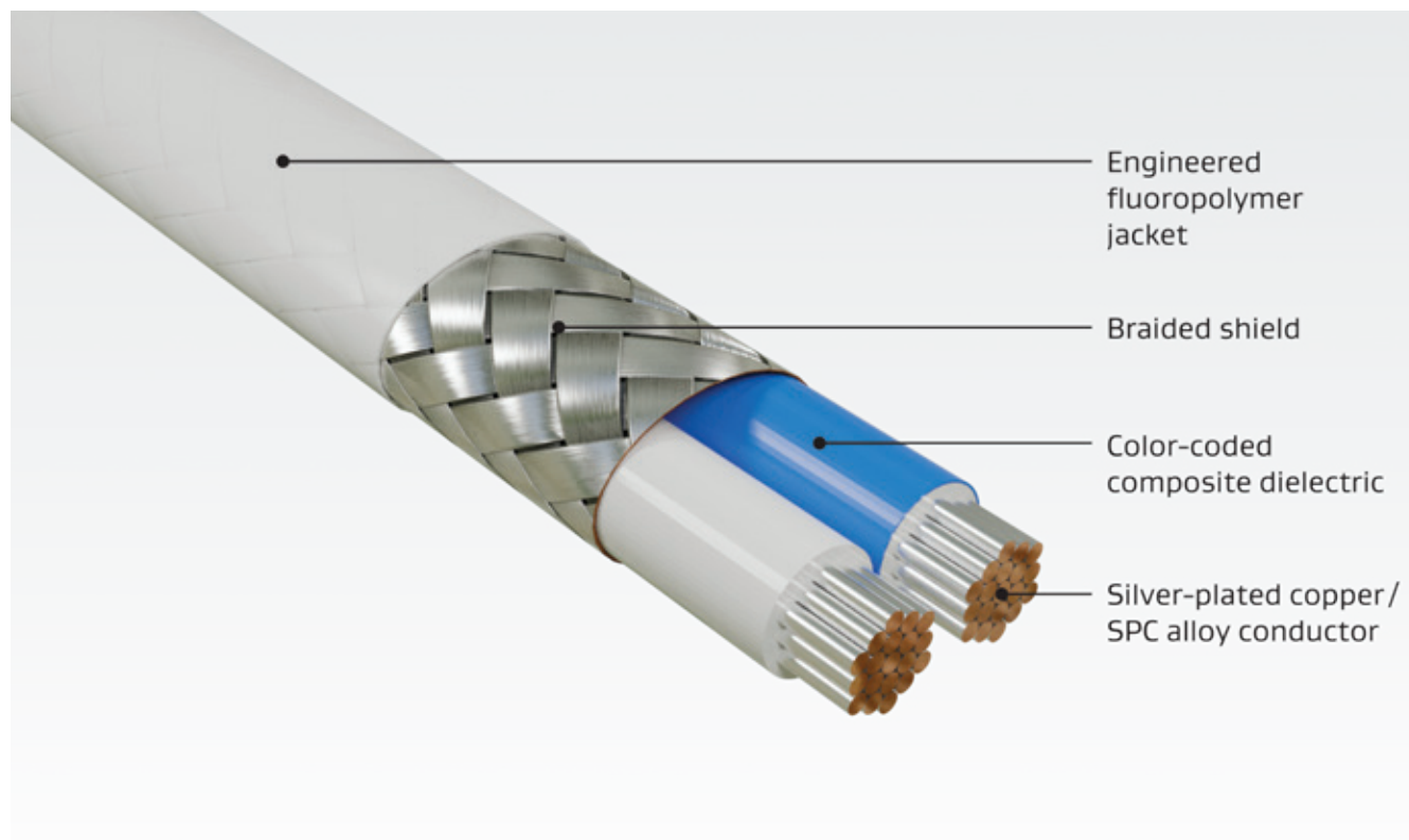
Figure 3: Durable Package
