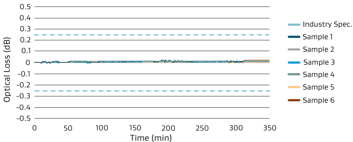
Figure 6: Vibration Endurance at +135°C (850 nm)
