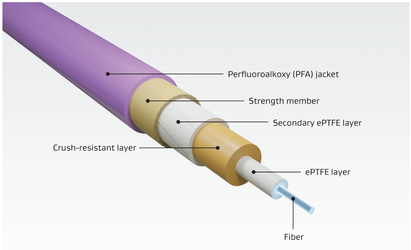
Figure 1: Crush-Resistant Layers
