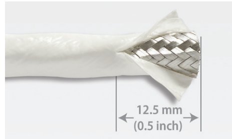
Figure 7: Peel-Back Method
