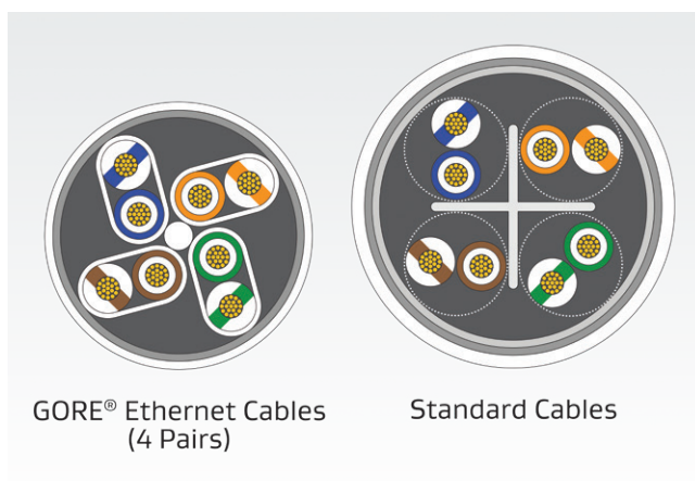
Figure 2: Reduced Diameter
