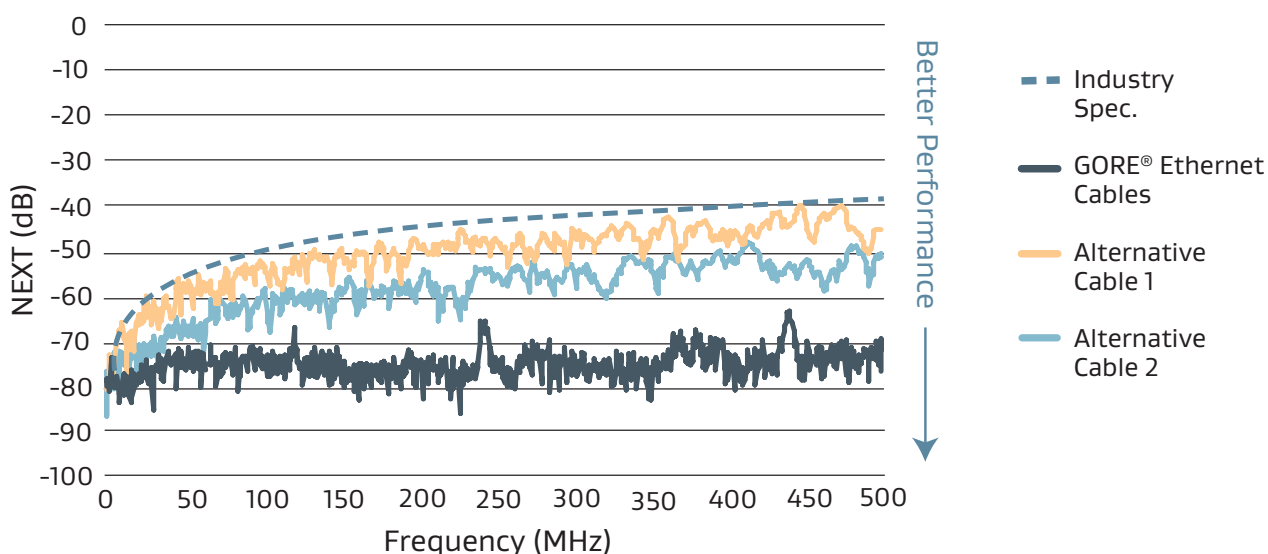
Figure 4: Crosstalk Comparison
