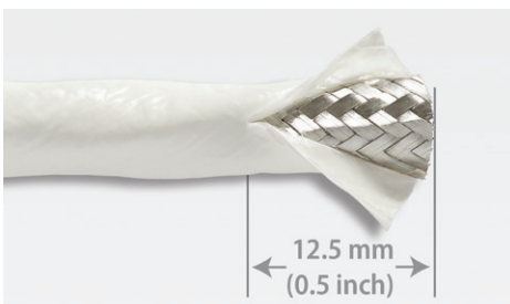
Figure 2: Peel-Back Method
