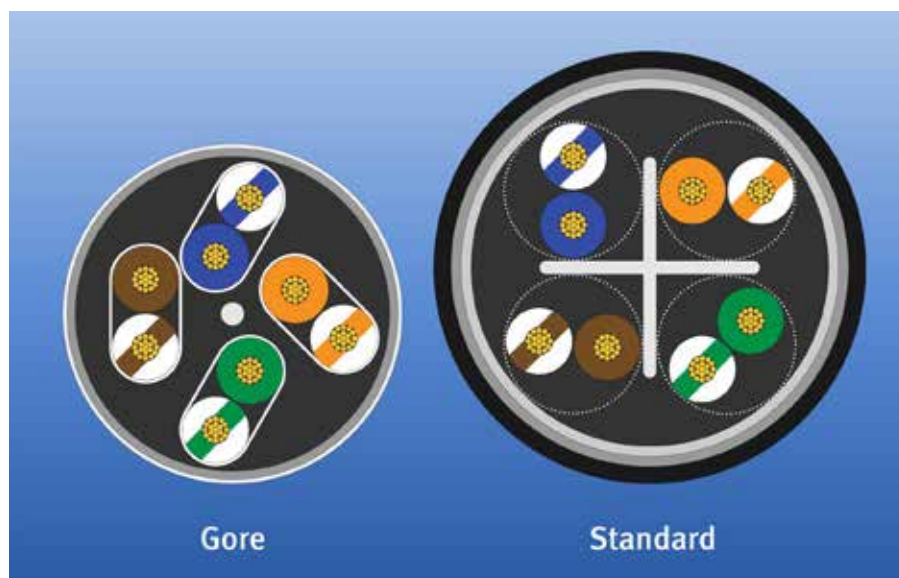
Figure 3: Comparison of Ethernet Cat6a Cable Designs
