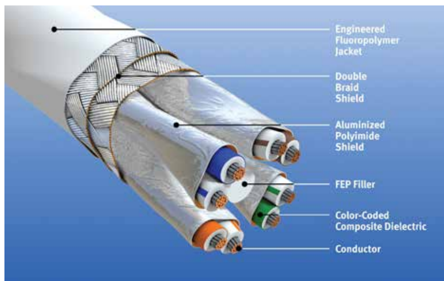
Figure 4: Construction of GORE® Ethernet Cables
