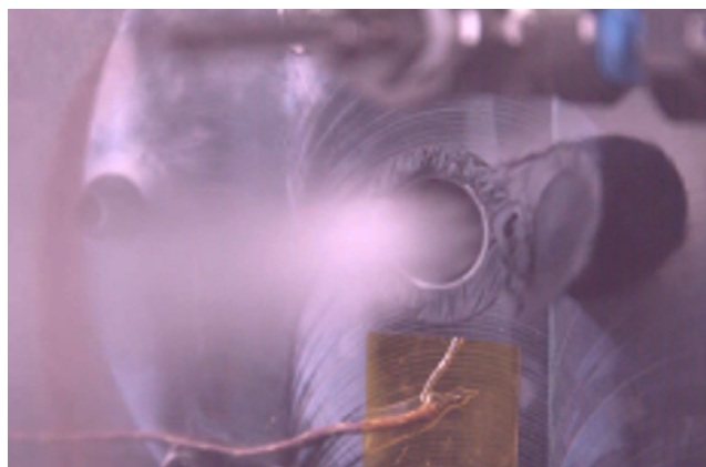
Figure 11: The cover plate after activation of GORE Vent, Thermal Runaway Test #1
