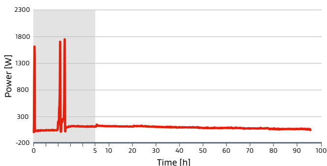
Power consumption
