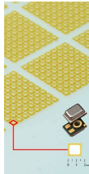
GORE® MEMS Protective Vents Style 200
