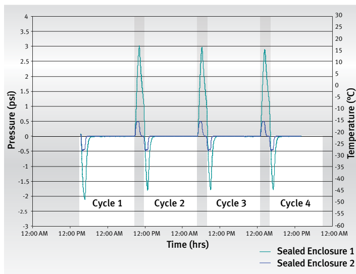
FIGURE 5: PRESSURE DIFFERENTIALS FOR SEALED ENCLOSURES
