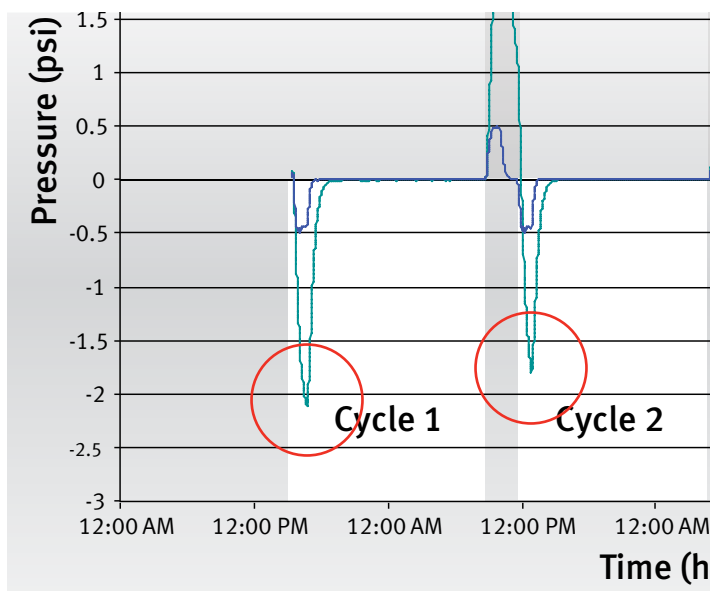
FIGURE 6: PRESSURE DIFFERENTIALS FOR FIRST SEALED ENCLOSURE
