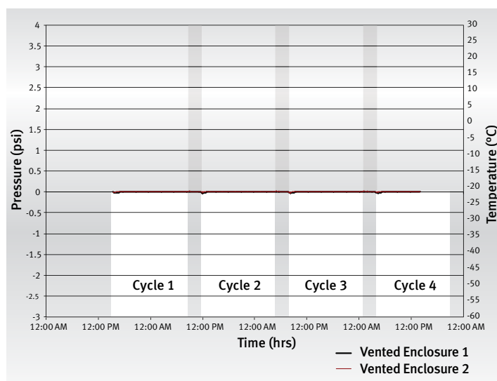
FIGURE 4: PRESSURE DIFFERENTIALS FOR VENTED ENCLOSURES
