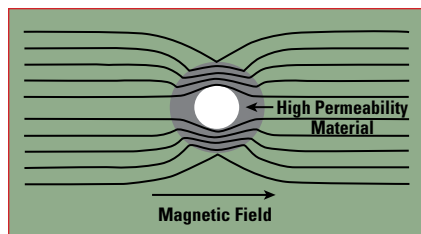
▲ Fig. 2 Magnetic field shielding.
