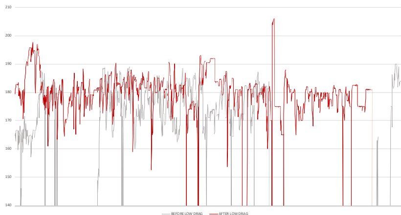
Figure 2. Cement plant #2 – BH Inlet pressure (mbar).
