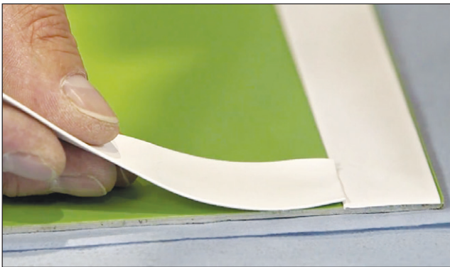
Figure 15: Sealing the two ends of the tape
