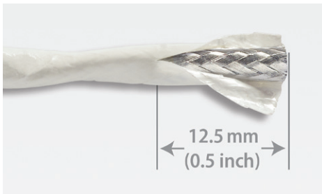
Figure 4: Peel-Back Method
