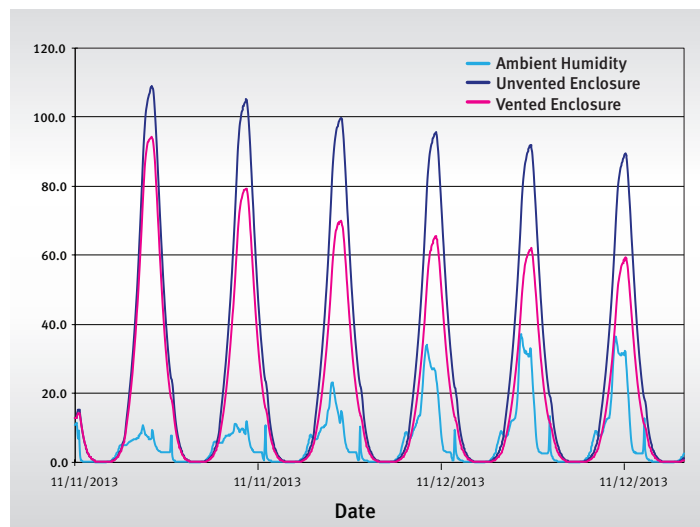
FIGURE 3: ABSOLUTE HUMIDITY
