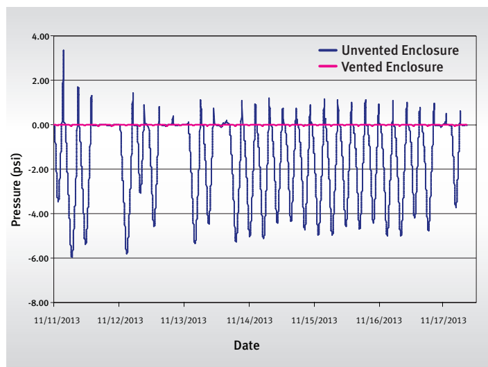
FIGURE 2: DIFFERENTIAL PRESSURE
