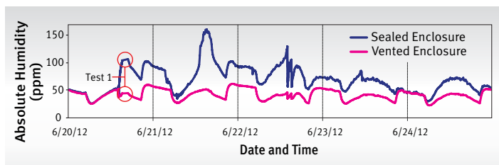
FIGURE 12: ABSOLUTE HUMIDITY DURING SHOCK TESTS
