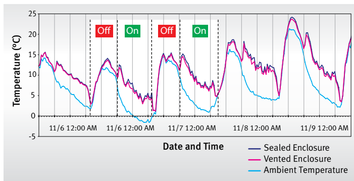
FIGURE 4: TEMPERATURE CYCLES
