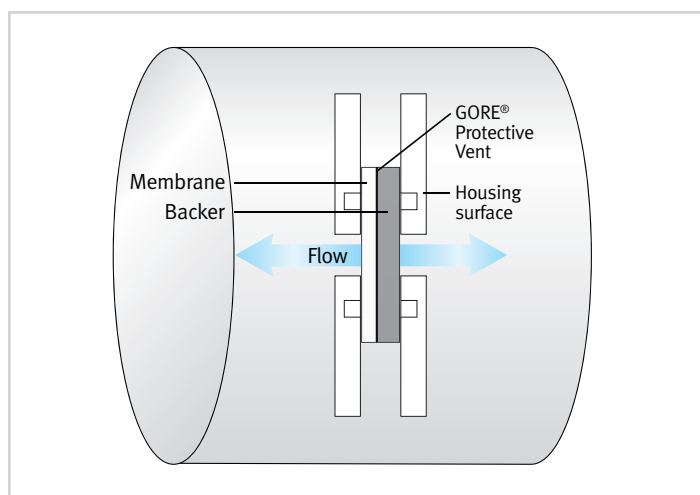
FIGURE 3: ADHESIVE VENT POSITION DURING AIRFLOW TEST
