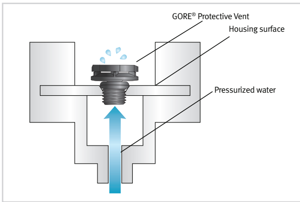
FIGURE 6: SCREW-IN VENT POSITION IN WATER PRESSURE TESTING EQUIPMENT
