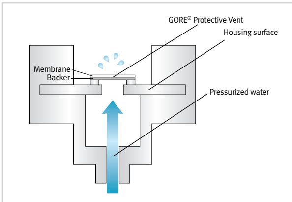
FIGURE 5: ADHESIVE VENT POSITION WITHIN WATER PRESSURE TESTING EQUIPMENT
