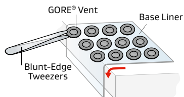
Figure 2: Manually dispensing an Adhesive Vent
