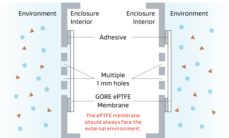
Figure 7: Interior or exterior mounting is recommended for Parts Series VE7 and VE9
