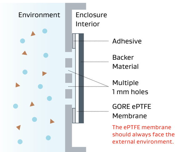
Figure 6: Interior mounting is recommended for Parts Series VE8
