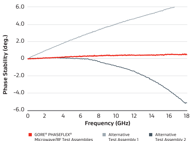
Figure 4: Phase Stability with Flexure of New Cables
