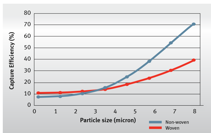
FIGURE 5: MODIFIED ASHRAE 52.2 TEST RESULTS FOR WOVEN AND NON-WOVEN MATERIALS
