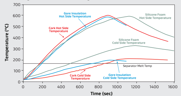
Figure 3: BESS Thermal Testing Data
