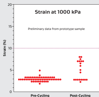
Figure 2: GORE Battery Insulation Compression Under High Stress and After Cyclic Loading Up to 2000 kPa
