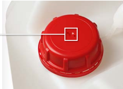
Venting hole Ø 2 ± 0,2mm
