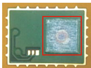
Figure 1: Typical placement of Style 200 on a MEMS PCB
