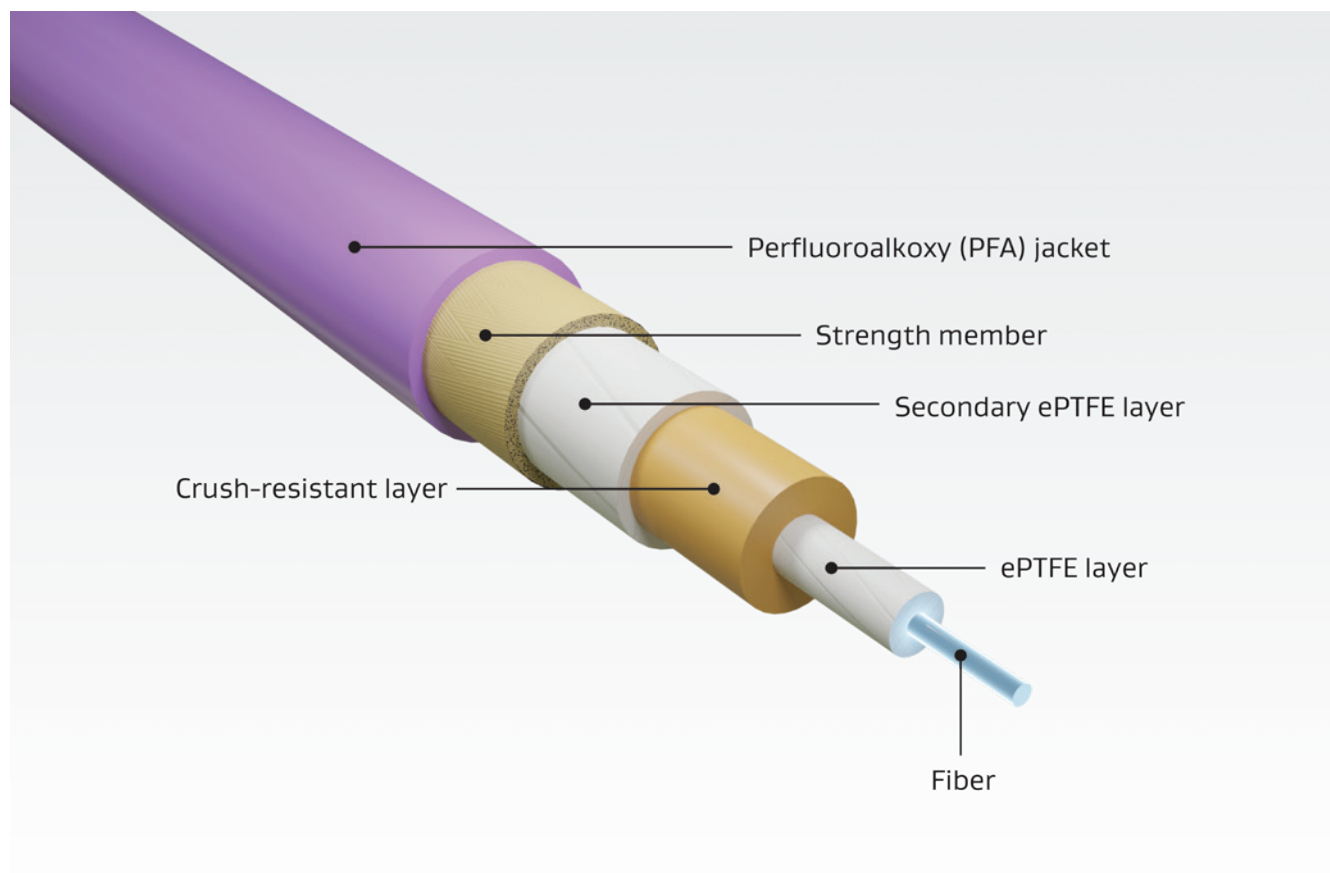
Figure 40: Crush-Resistant Layers
