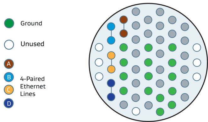
Figure 34: MIL-DTL-38999, Size 21 Non-Optimized Pinout Video Configuration
