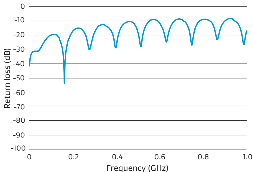
Figure 28: Return Loss Performance
