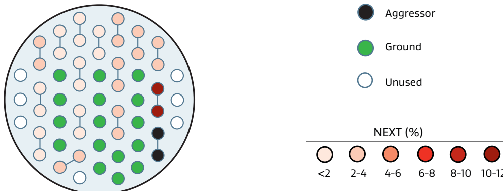
Figure 21: Aggressor Signal at bG
