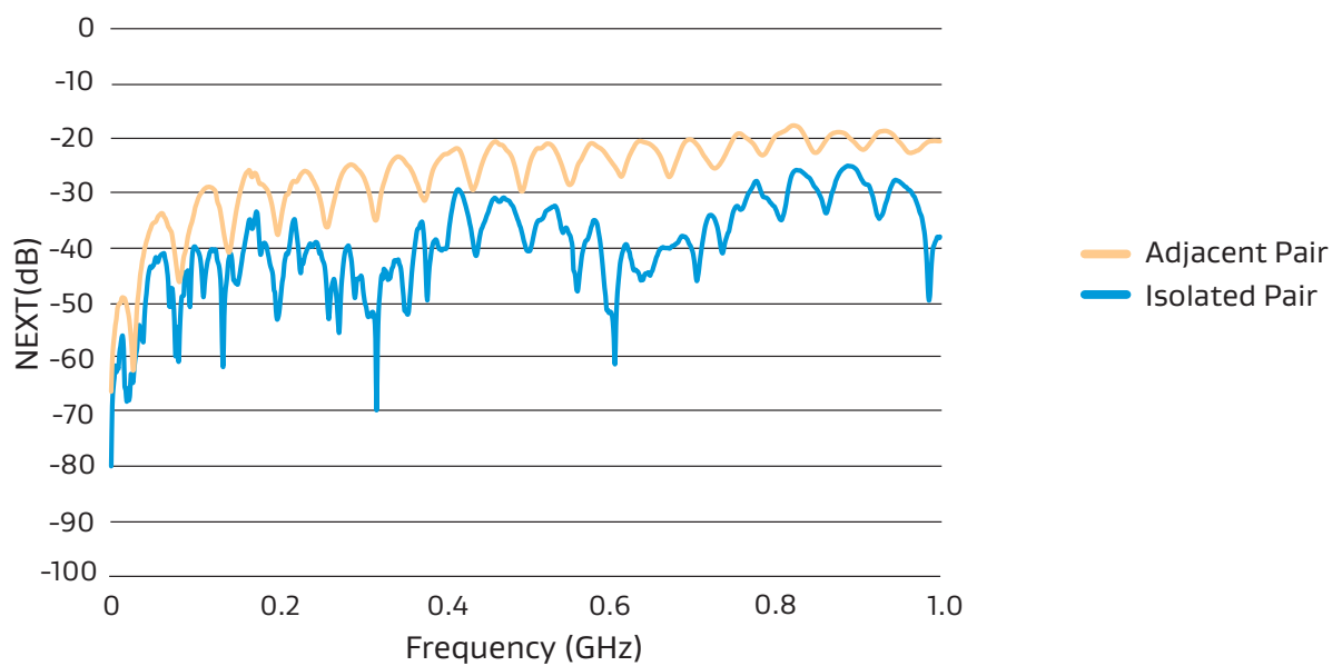
Figure 16: Crosstalk Performance for Adjacent Pair and Isolated Pair
