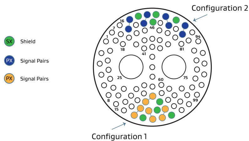
Figure 35: SAE AS6129 Optimized Pinout Configuration
