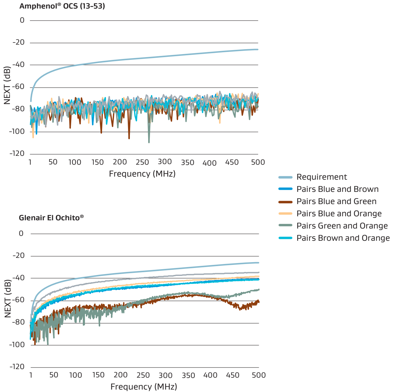
Figure 9: Crosstalk Comparison of Ethernet Cables
