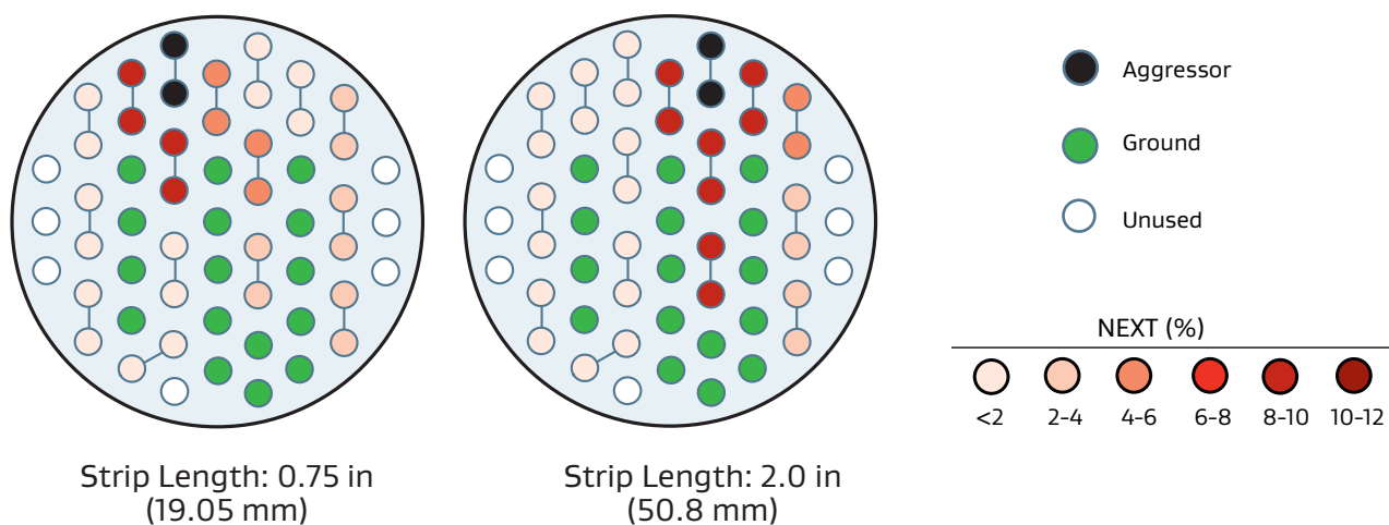
Figure 22: Crosstalk Comparison between Pairs
