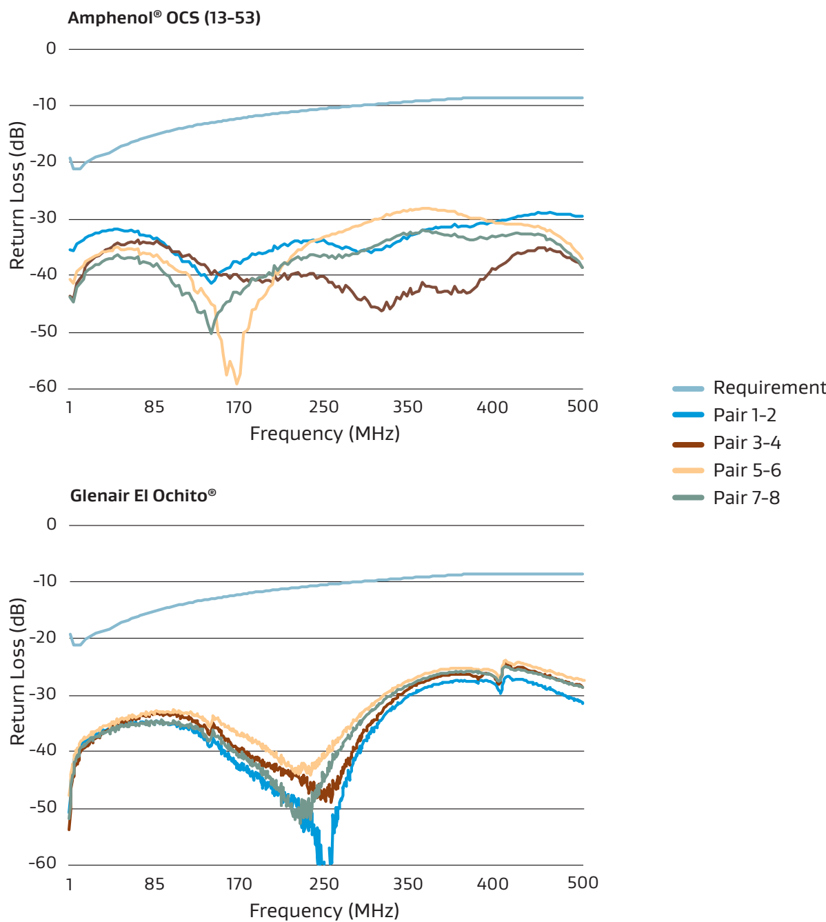
Figure 8: Return Loss Comparison of Ethernet Cables
