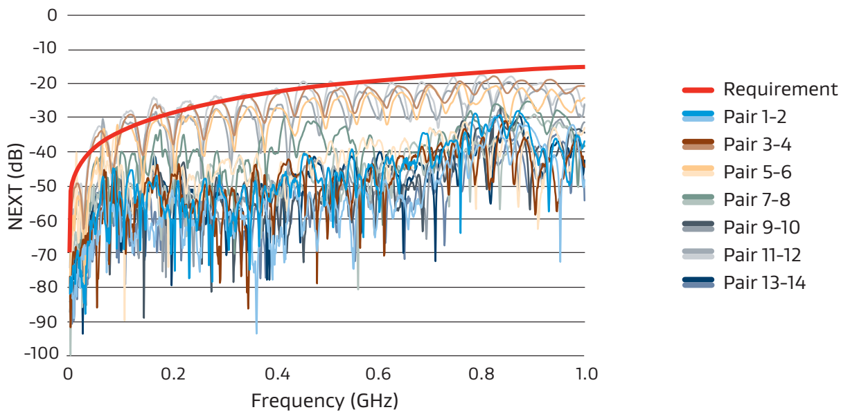
Figure 15: Crosstalk Limit Lines Performance between Victim and Other Pairs (15 Interactions)
