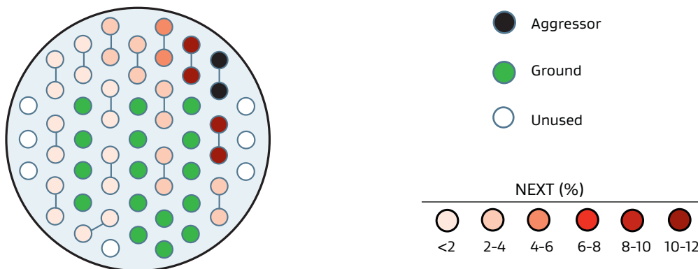
Figure 19: Aggressor Signal at CY
