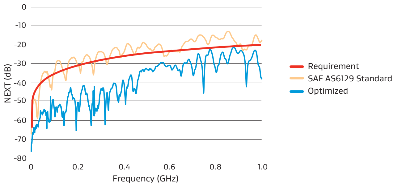
Figure 32: Worst-Case Crosstalk Comparison for Standard and Optimized Pinout Configurations
