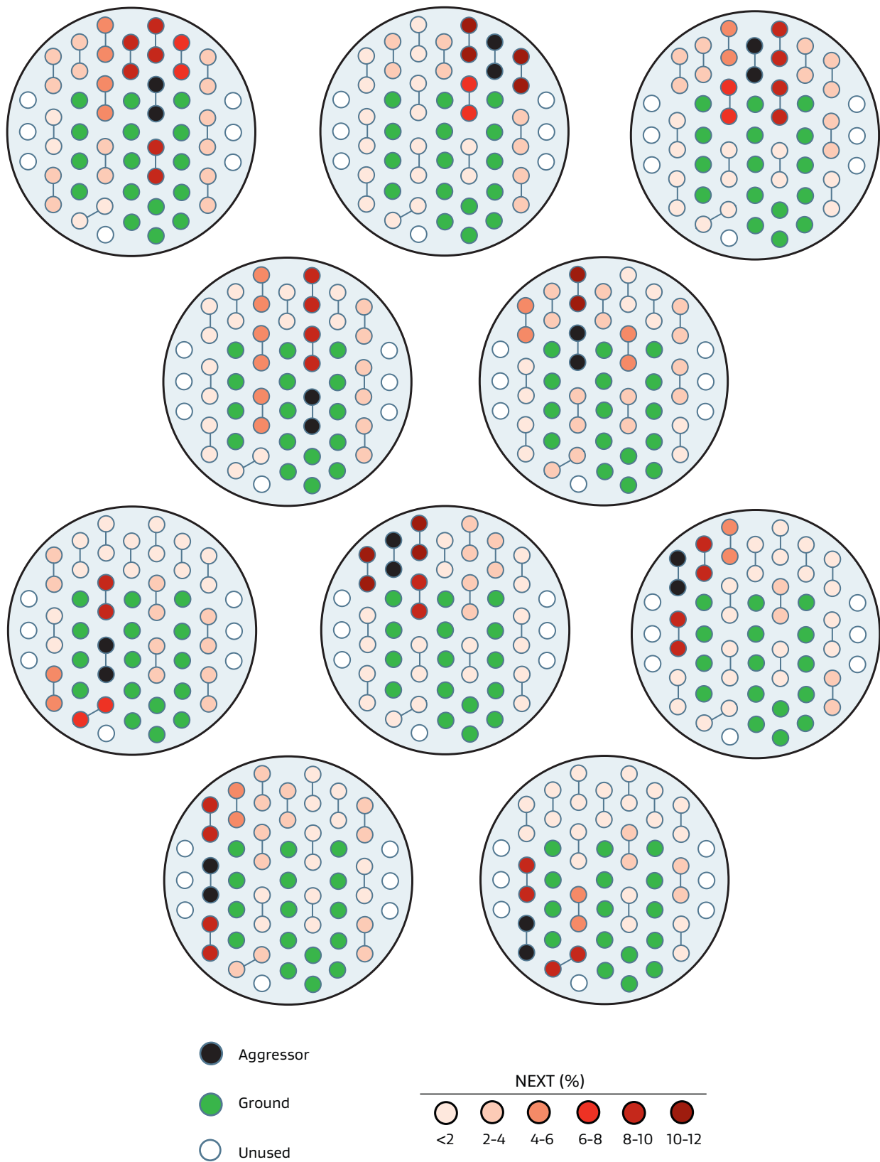
Figure 23: Crosstalk Mapping for Remaining Victims in the MIL-DTL-38999 Open Pin Field Connector System
