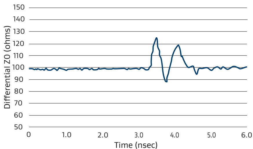
Figure 27: Characteristics Impedance Traces through Connector Interface
