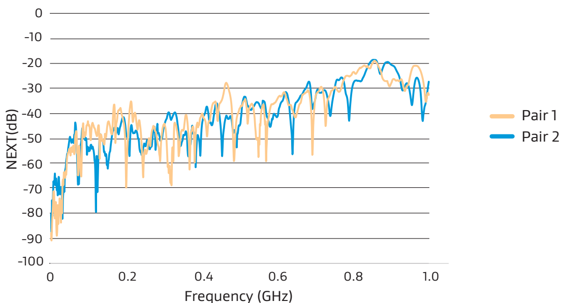
Figure 17: Crosstalk Performance for 2 Sets of Pairs
