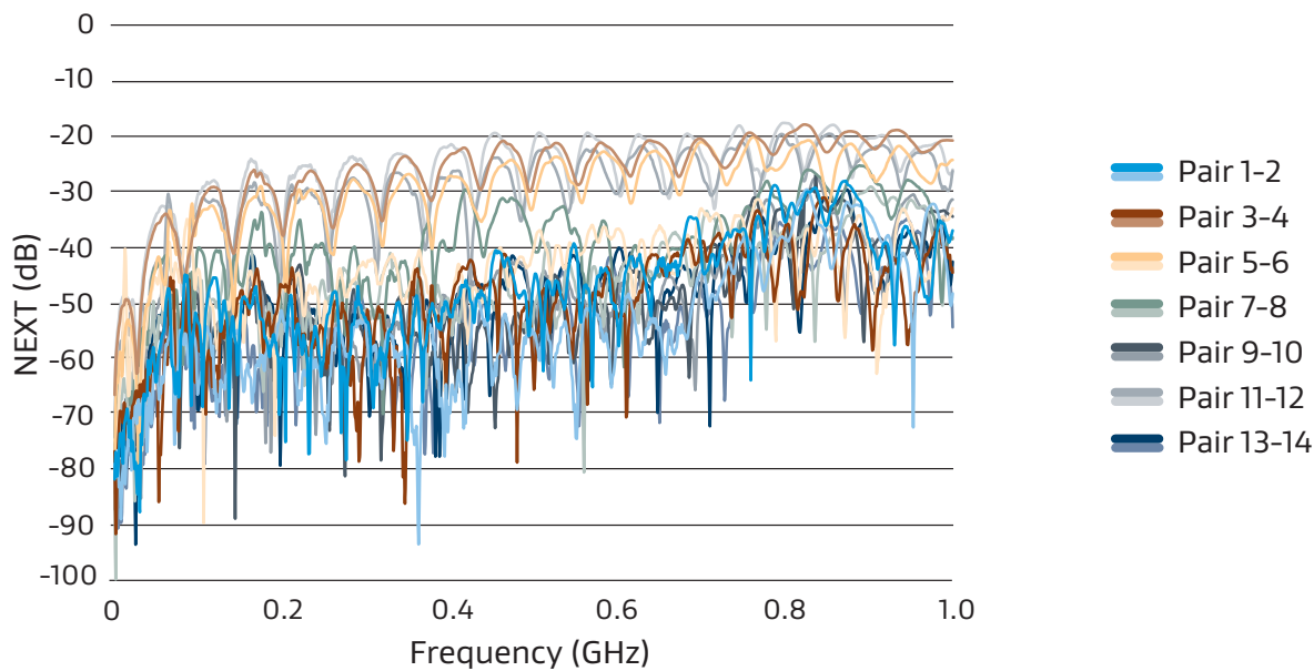
Figure 14: Crosstalk Performance between Victim and Other Pairs (15 Interactions)
