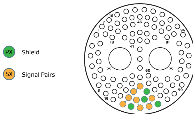
Figure 26: Pin Configuration Defined in SAE AS6129
