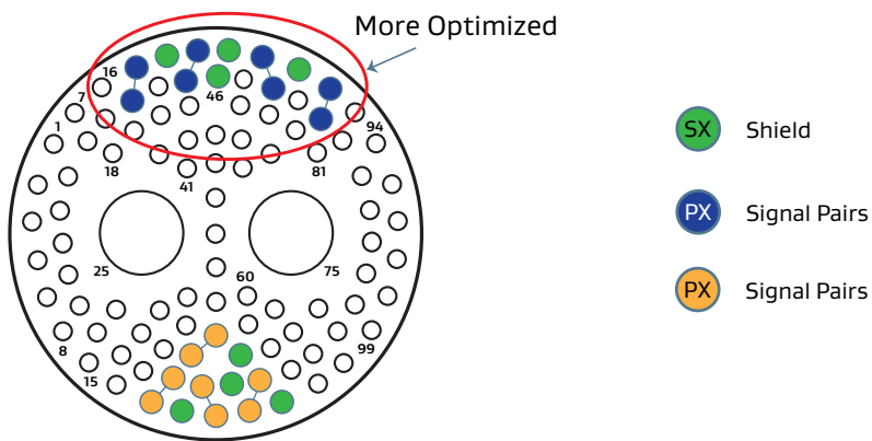
Figure 30: SAE AS6129, Size 25 Optimized Pinout Configuration
