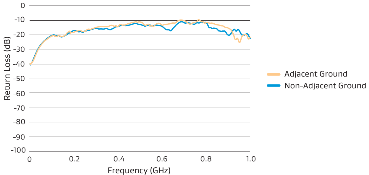
Figure 12: Return Loss for Adjacent and Non-Adjacent Shield Connections
