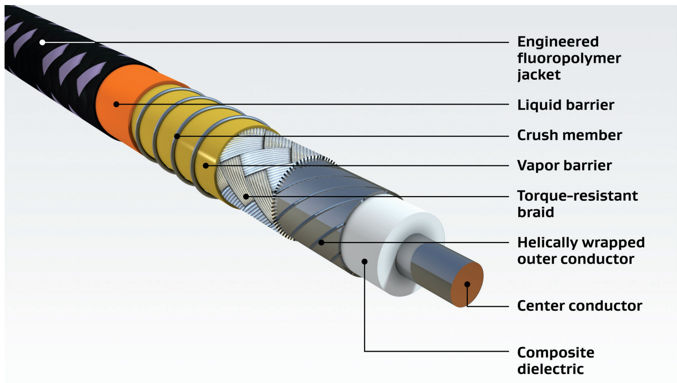
Figure 4: Rugged Construction of GORE-FLIGHT™ Microwave Assemblies, 6 Series
