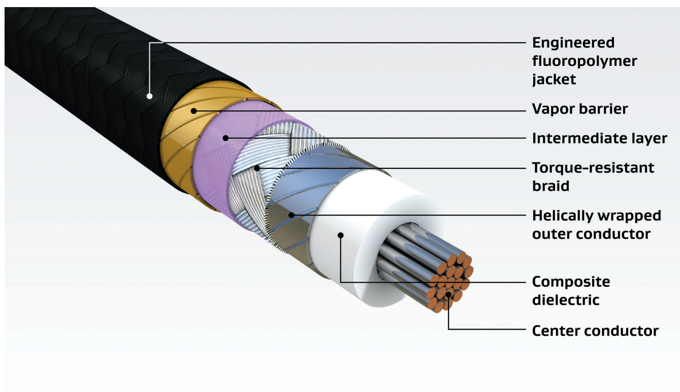
Figure 3: Vapor-Sealed Construction of GORE® Microwave/RF Assemblies, 7 Series
