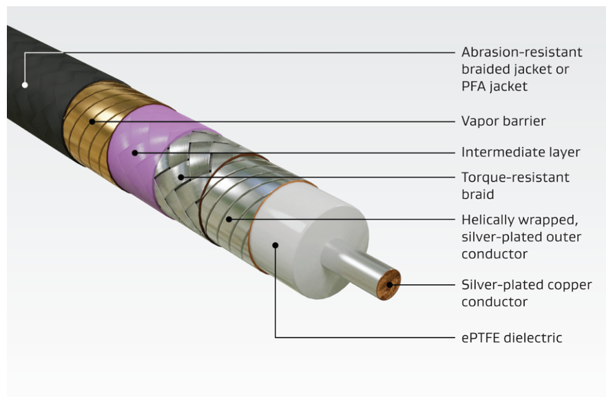
Figure 10: Vapor-Sealed Construction
