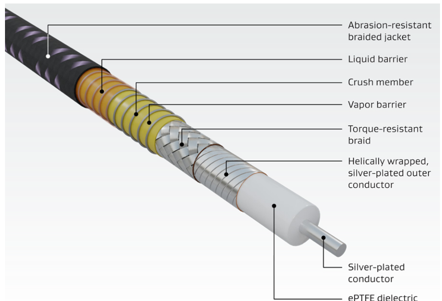
Figure 3: Rugged Construction
