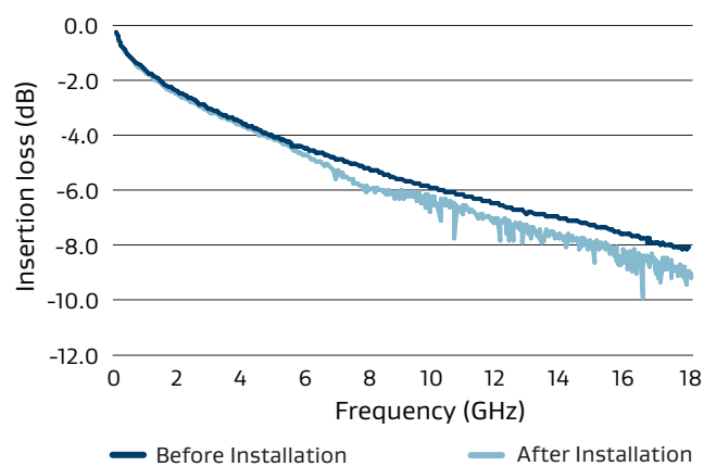
Figure 7: Leading Competitor Assembly Insertion Loss
