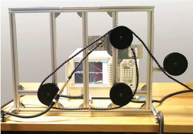
Figure 7: Installation Simulator
