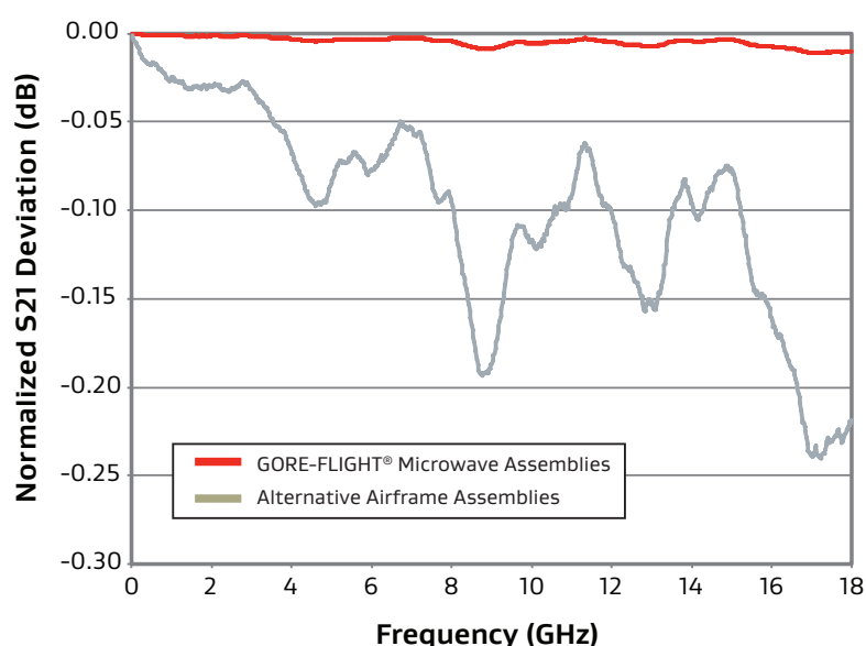
Figure 5: Shake stability results of cable assemblies
