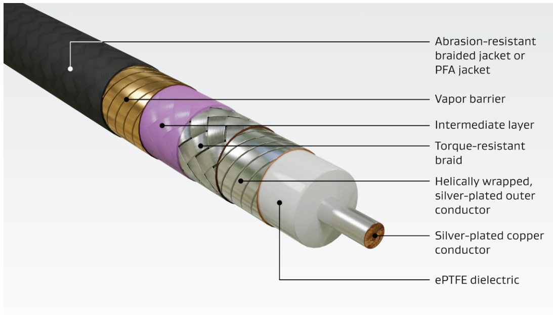
Figure 6: Cable Construction
