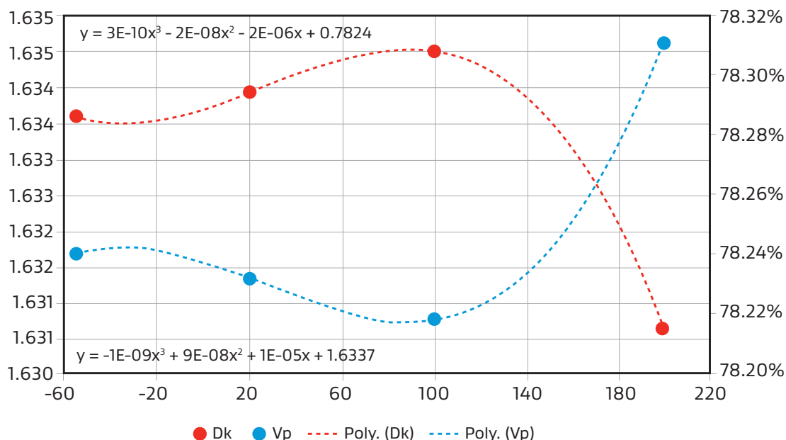
Figure 1: Performance Results for Dielectric Properties over Temperature
