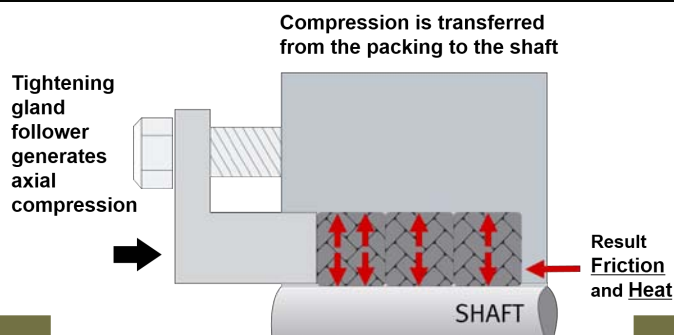
Figure 3. Sealing forces and packing
