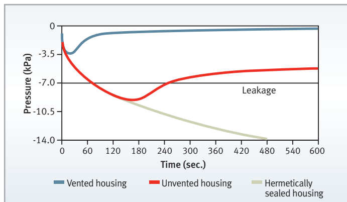
FIGURE 1: INTERNAL PRESSURE OF VENTED AND UNVENTED HOUSINGS
