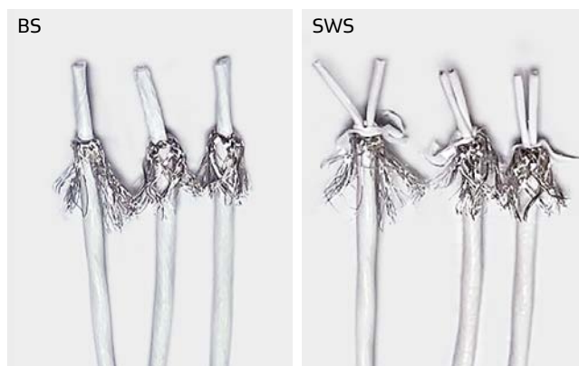
Figure 2: Test specimens from W. L. Gore & Associates
