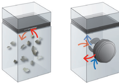
Unvented: Failed seals let contaminants enter the housing
