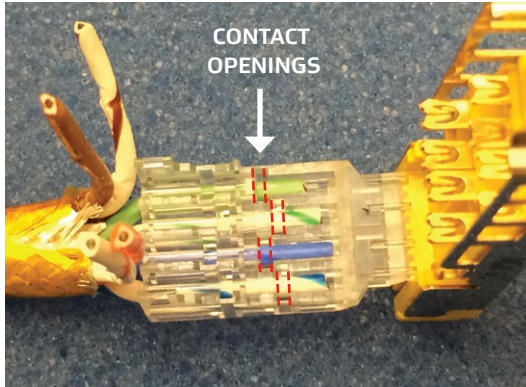
Figure 11: Wires inserted in position in bottom row
