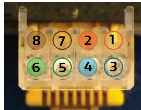
Figure 9: Wire positions inside connector
