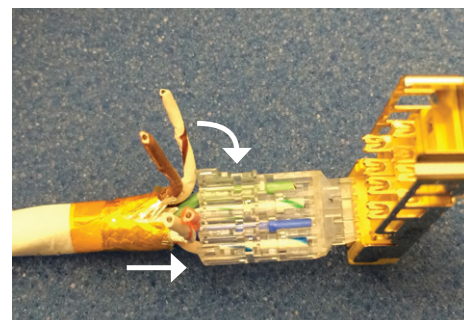
Figure 10: Inserting wires in bottom row
