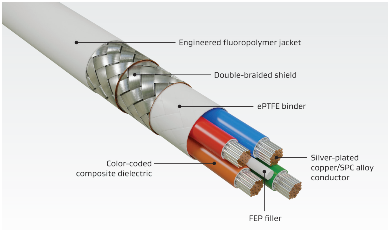
Figure 1: Highly Flexible Cable Technology
