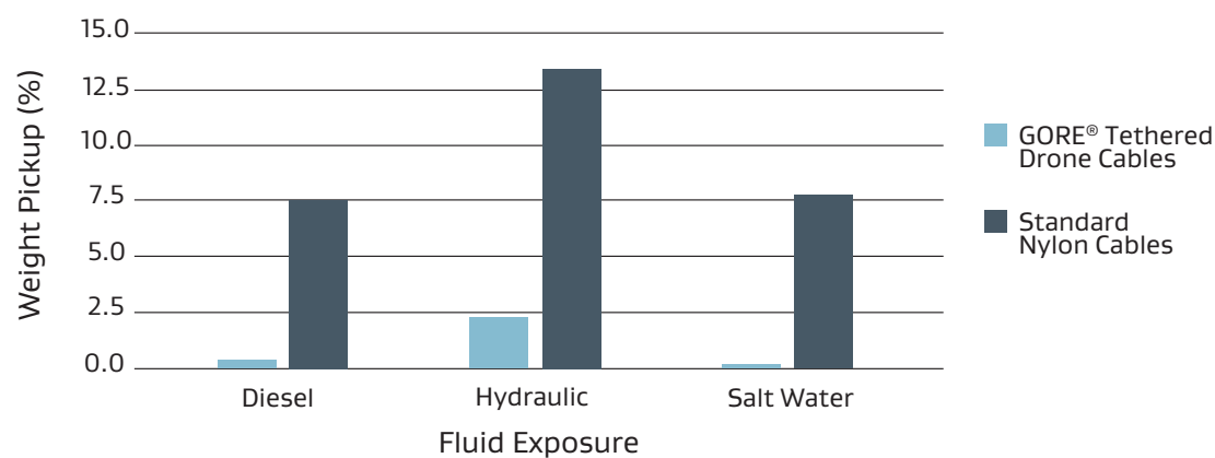
Figure 5: Fluid Resistance Comparison of Tethered Drone Cables
