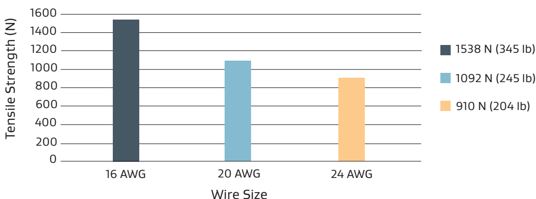
Figure 4: Tensile Strength of GORE® Tethered Drone Cables
