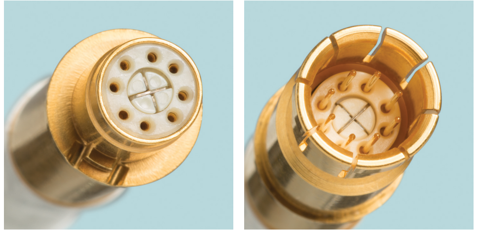
Figure 6: Glenair El Ochito® — Multi-pin Insert (size 8) Connector
