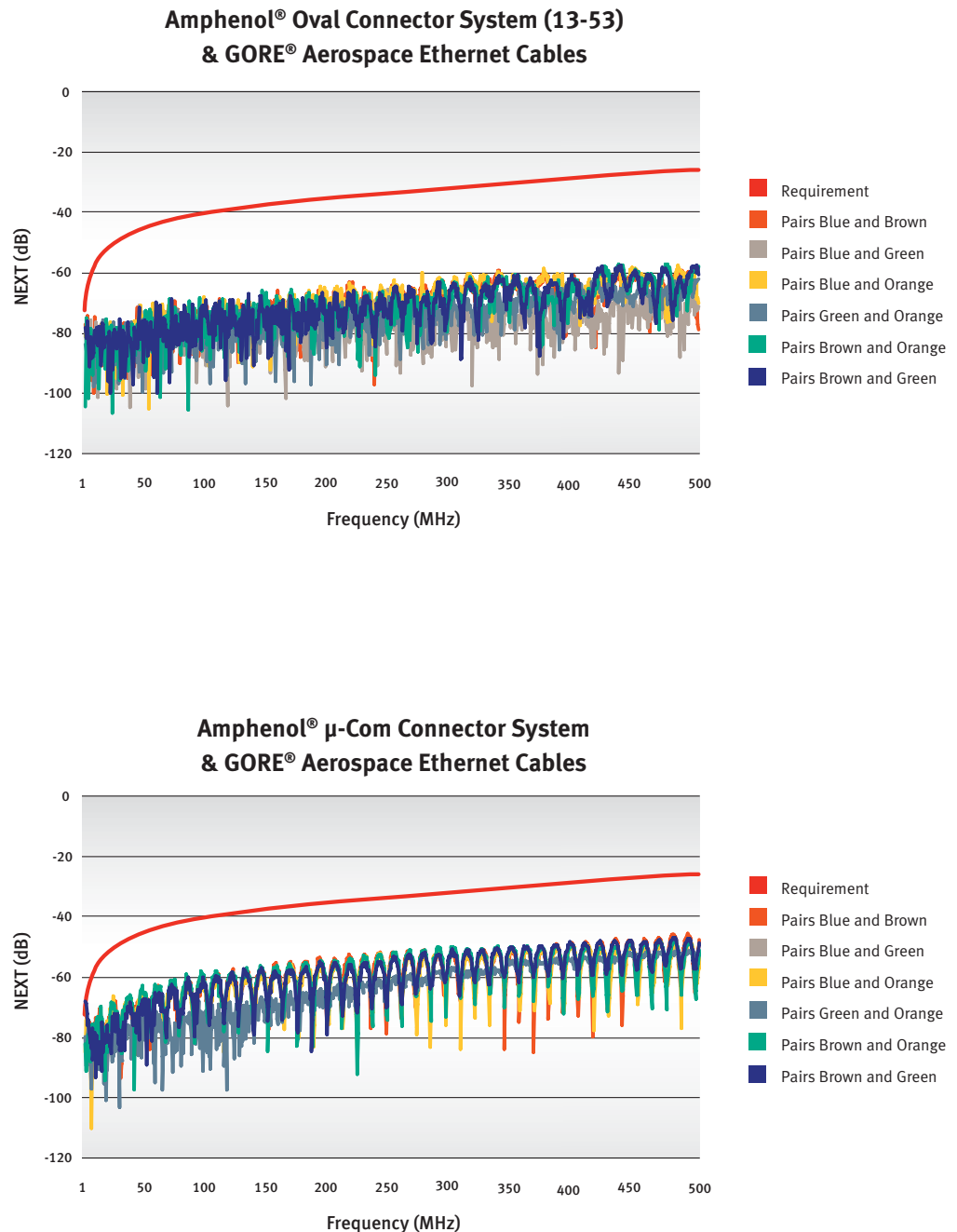
Figure 15: Near-End Crosstalk (NEXT) of Ethernet Interconnects
