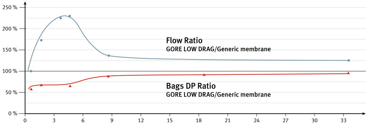
FLOW RATIO: GORE® LOW DRAG™ FILTER BAGS VS. STANDARD BAGS (NEW)
