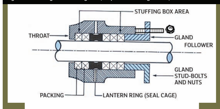
Figure 1. Packing in a stuffing box (Graphics courtesy of FSA)
