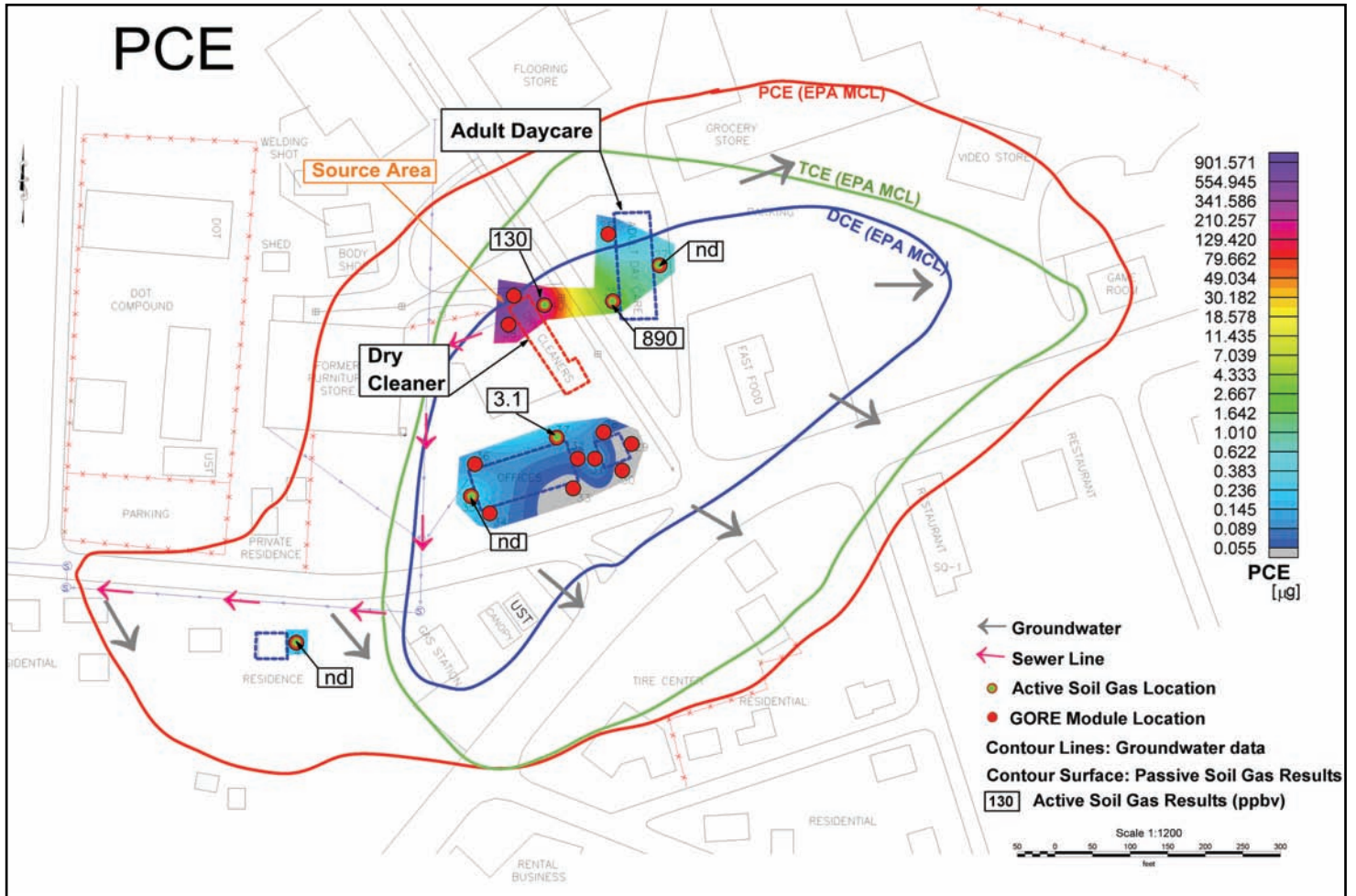
Figure 1. Passive soil gas results contoured (µg) with active soil gas results posted (ppbv).
