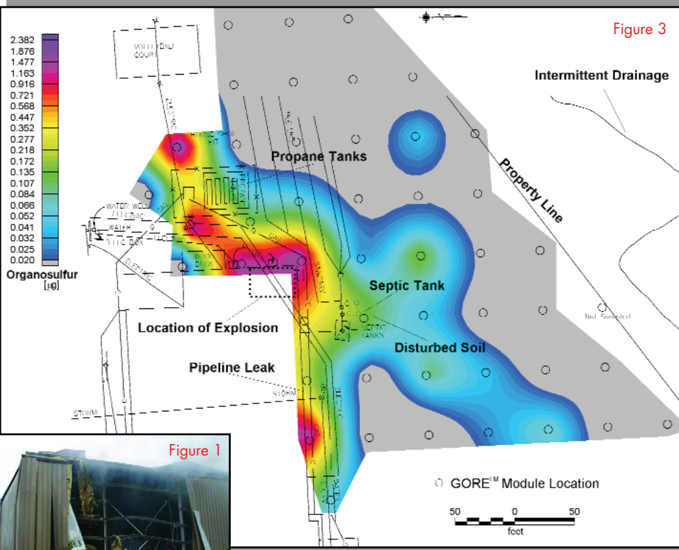
Figure 1: Warehouse Figure 2: Delineation of propane in soil gas. Figure 3: Delineation of organosulfur compounds in soil gas.
